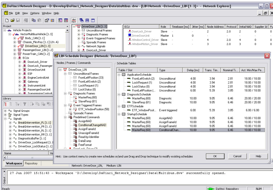
Designing the LIN schedule with DaVinci Network Designer LIN
