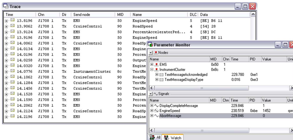
Protocol-specific representation in the Trace Window, the Parameter Monitor displays all sent PIDs of a MID
