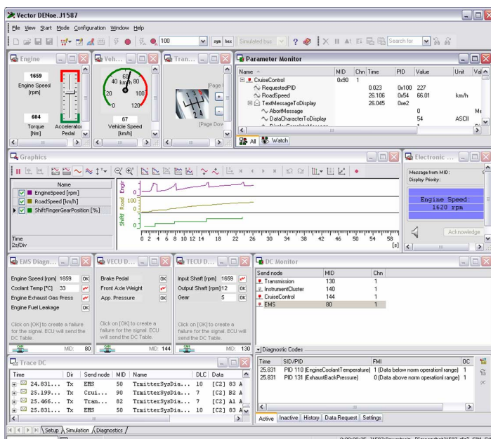
CANoe.J1587 configuration with Parameter Monitor, Diagnostic Monitor and panels
